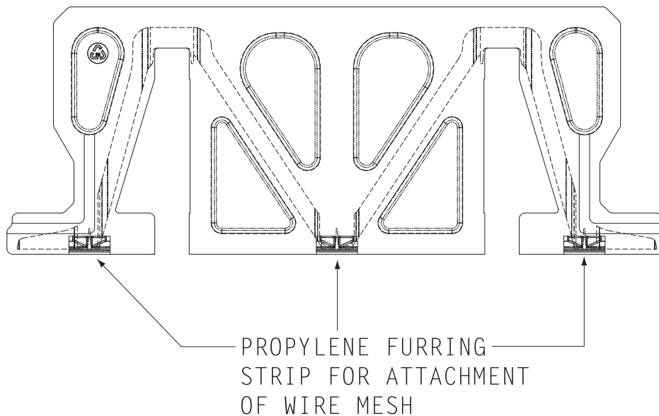
Figure 9.2 - Furring strips on AmDeck™
