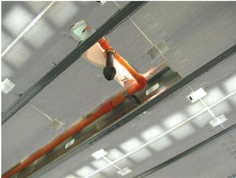
Figure 6.4 – Large pipe attached to steel joist
