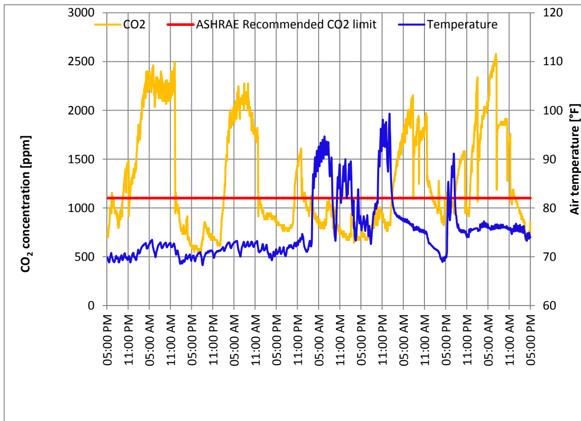
Figure 19. Temperature and CO 2 concentration in a Spruce house bedroom. The bedroom is above the ASHRAE recommended 1100 ppm most of the time the room is occupied.
