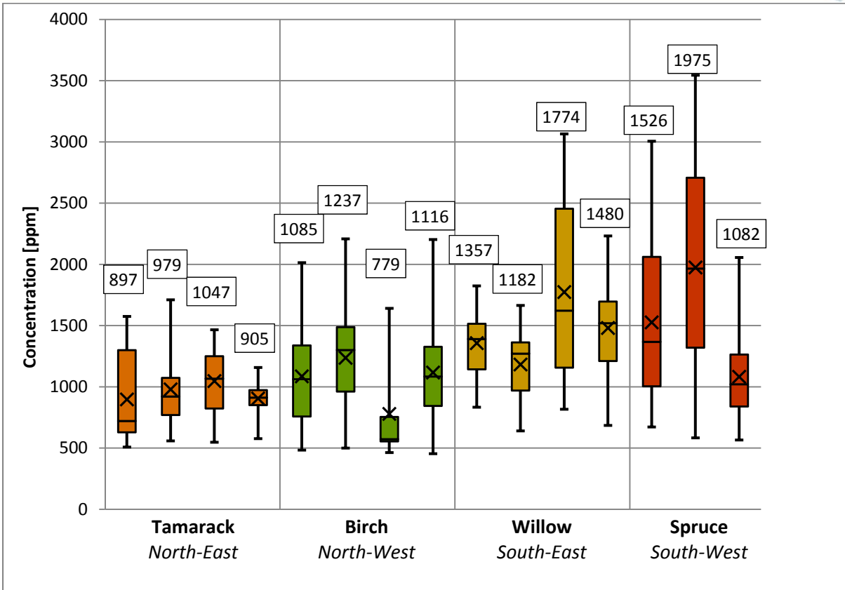
Figure 15. CO 2 concentrations in bedrooms during the night hours (10:00 p.m. - 8:00 a.m.). The colored boxes describe the lower and upper quartiles, the bands inside the boxes are medians, crosses are mean values and the ends of the whiskers represent 1 st and 99 th percentiles.
