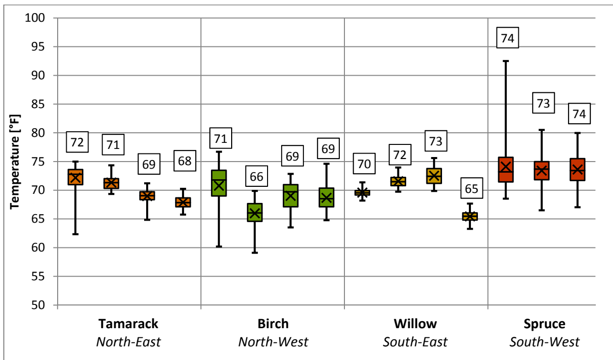
Figure 11. Temperature distribution in bedrooms. The colored boxes describe the lower and upper quartiles, the bands inside the boxes are medians, crosses are mean values and the ends of the whiskers represent 1 st and 99 th percentiles.
