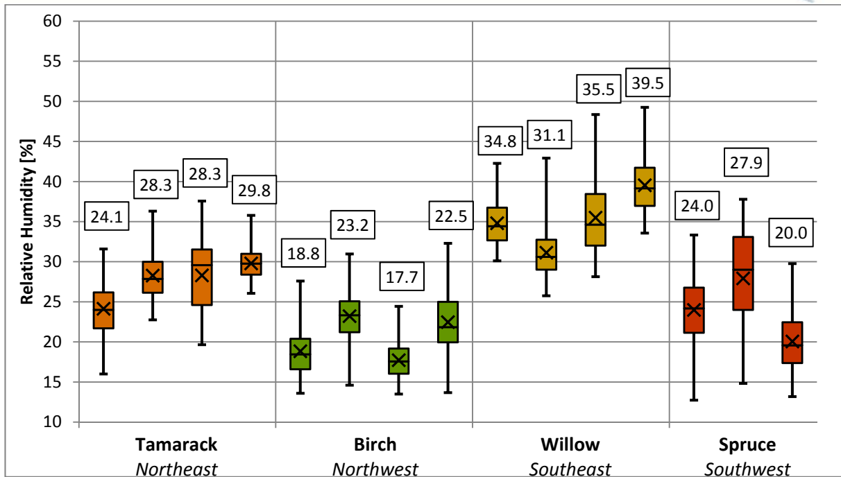
Figure 14. Relative humidity in monitored bedrooms. The colored boxes describe the lower and upper quartiles, the bands inside the boxes are medians, crosses are mean values and the ends of the whiskers represent 1st and 99th percentiles.
