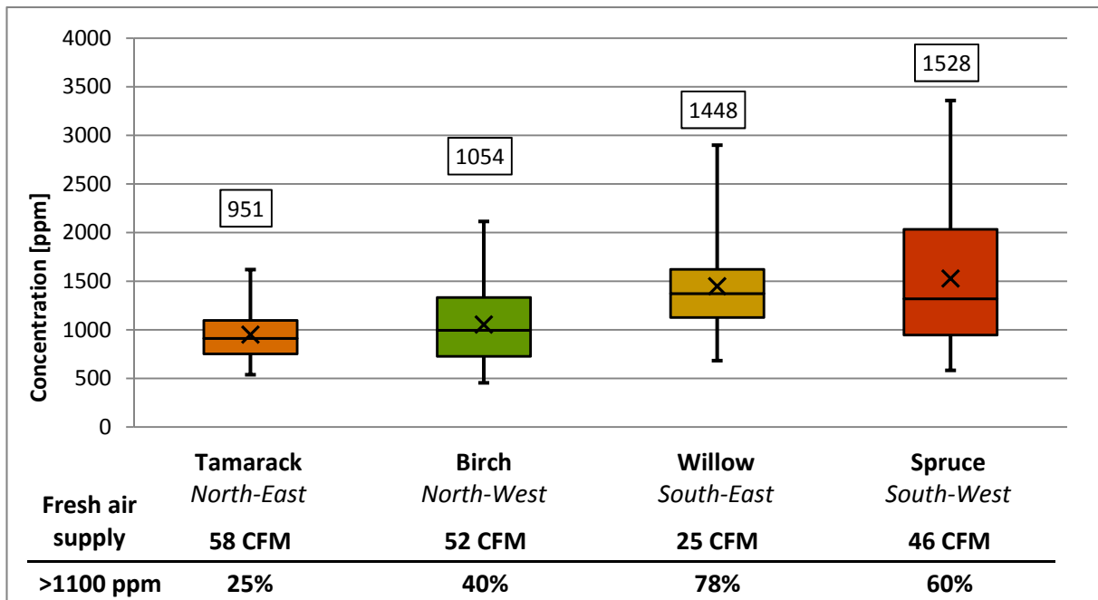
Figure 17. Night CO 2 concentrations for each house when all occupied bedrooms within the house are put together.
