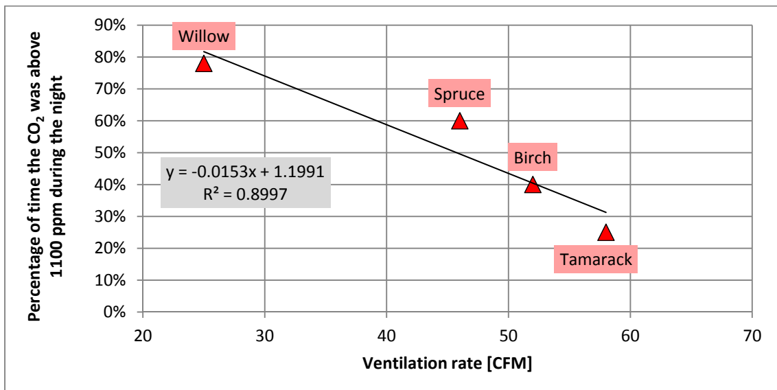
Figure 16. Ventilation rate vs. CO 2 concentration above the ASHRAE 1100 ppm limit
