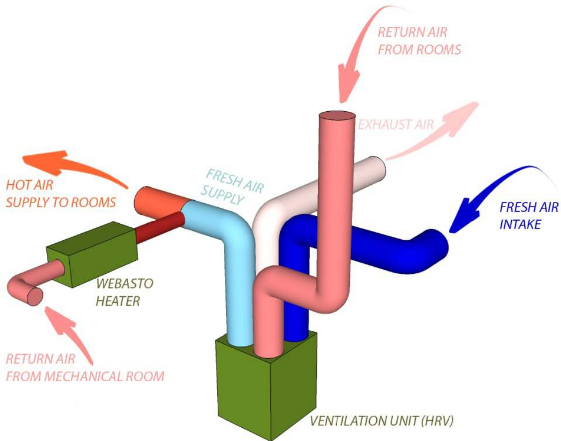
Figure 5. BrHEAT system schematic. The Webasto heater is an oil heater designed to heat commercial-sized truck cabins so the trucks wouldn't have to idle overnight to keep the cab warm.
