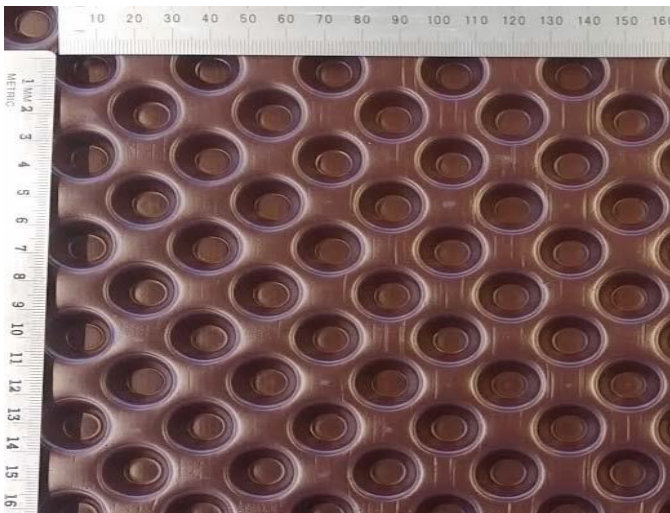
Figure 1. “DELTA®-MS” drainage membrane – face in contact with the soil
