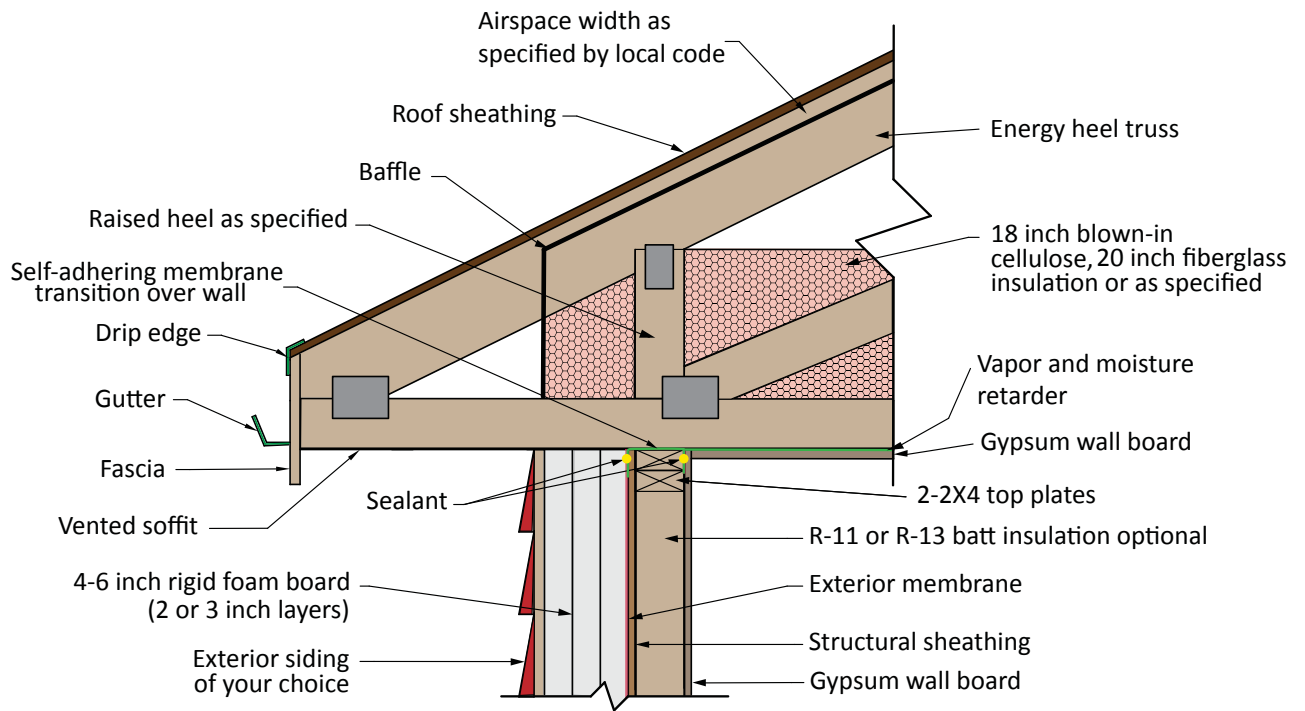
Figure 2. BRACING WITH ROOF INSULATION OVER WALL INSULATION
