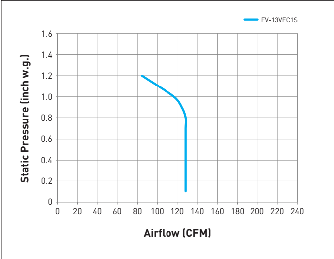
FV-13VEC1S Net Supply
