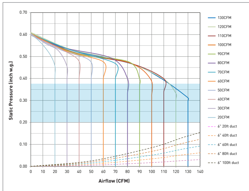
FV-13NLFS1 20-130 CFM 6" Duct
