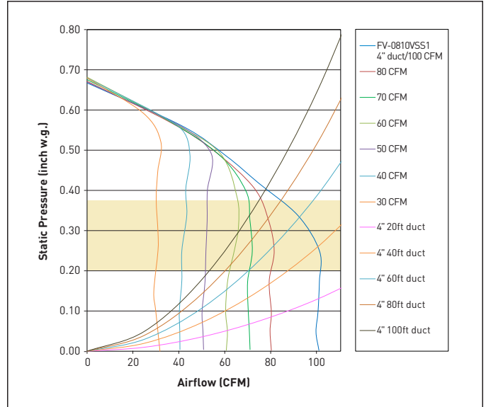
FV-0810VSS1 80-100 CFM 4" Oval Duct
