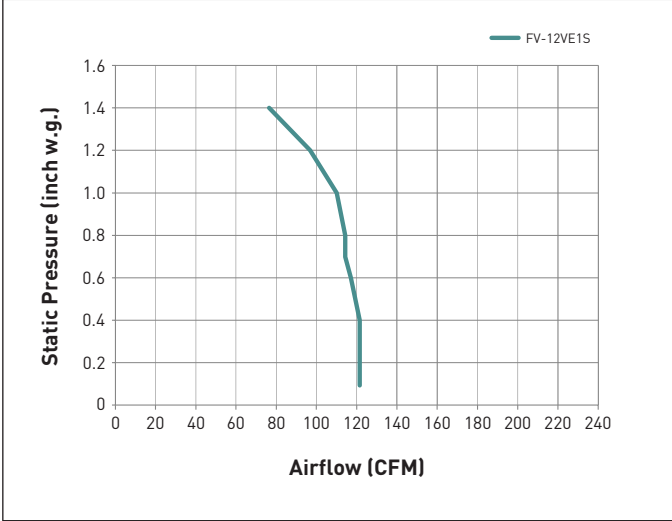
FV-12VE1S Net Supply
