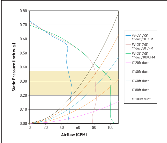
FV-0510VS1 50-80-100 CFM 4" Oval Duct
