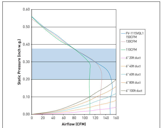
FV-1115VQL1 110-130-150 CFM 6" Duct
