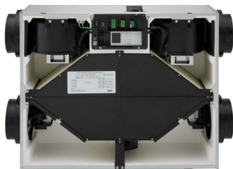
Elite Plus+ Cover Off
