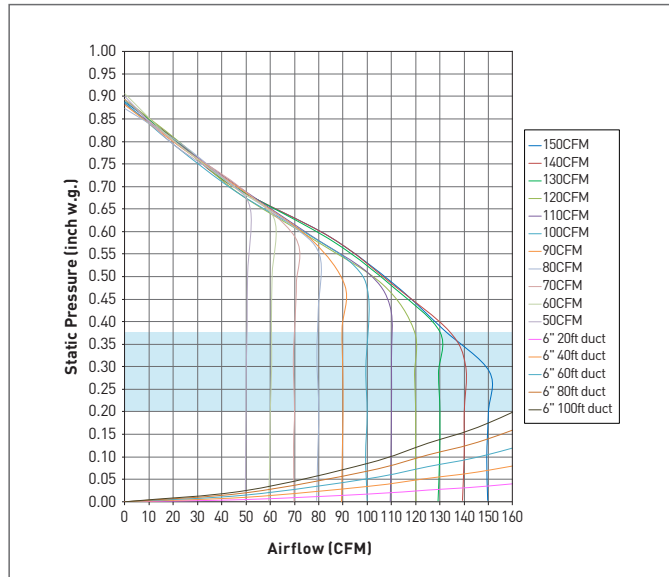
FV-15NLFS1H 50-150 CFM 6" Duct
