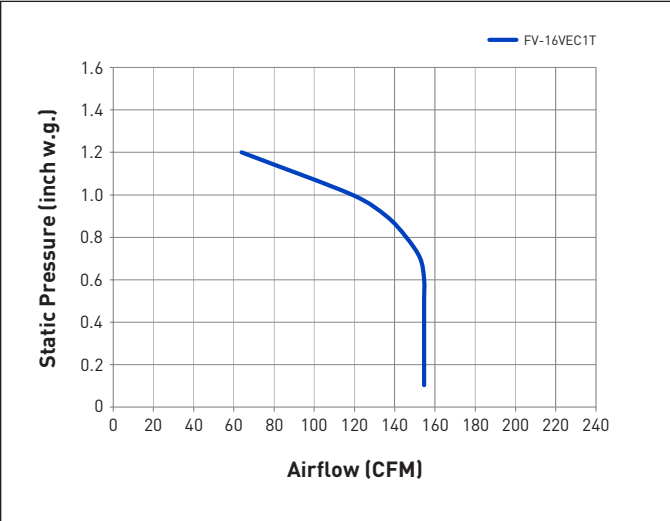
FV-16VEC1T Net Supply
