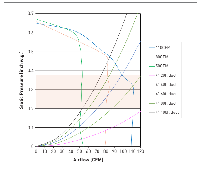
FV-0511VHL1 110 CFM 4" Duct
