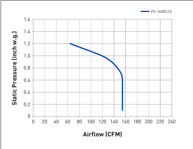
FV-16VEC1S Net Supply
