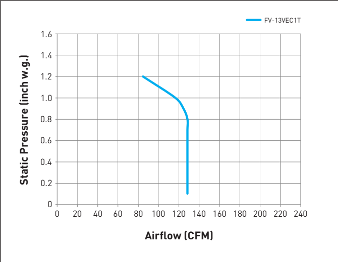
FV-13VEC1T Net Supply
