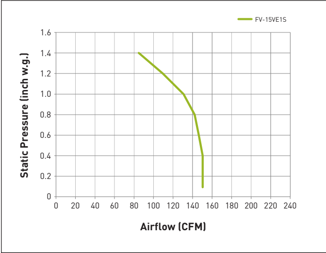
FV-15VE1S Net Supply
