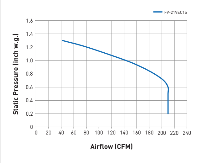
FV-21VEC1S Net Supply
