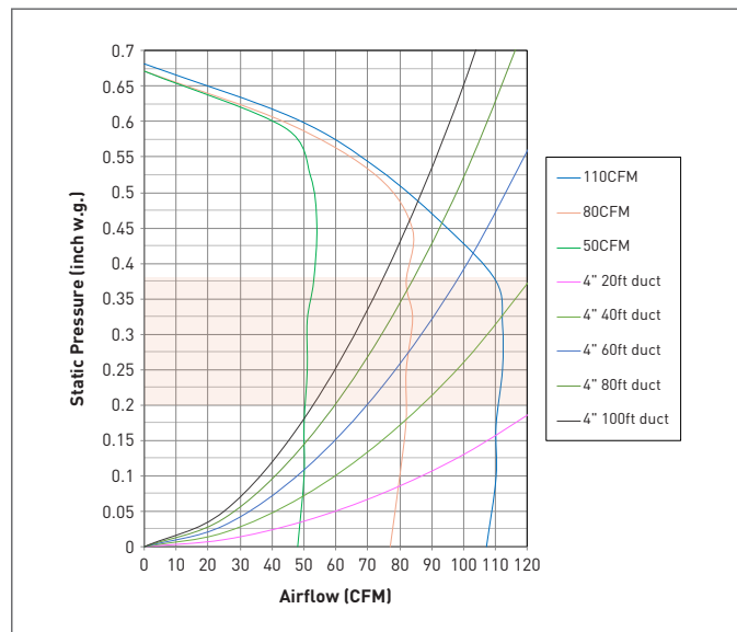
FV-0511VH1 110 CFM 4" Duct
